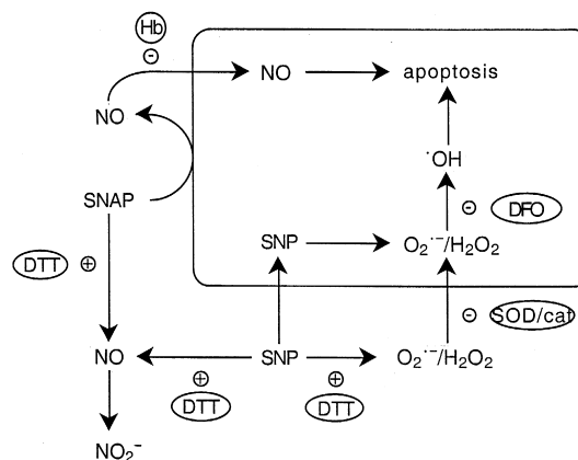
Fig. 10. Schematic representation of production of reactive oxygen species by sodium nitroprusside (SNP) and S -nitroso- N -acetylpenicillamine (SNAP) in the presence of cells, with and without dithiothreitol (DTT), leading to apoptosis. Places where different agents influence the decomposition or inhibit the action of sodium nitroprusside and S -nitroso- N -acetylpenicillamine are indicated. Dithiothreitol accelerates the decomposition of S -nitroso- N -acetylpenicillamine and sodium nitroprusside. Hemoglobin (Hb) blocks the action of S -nitroso- N -acetylpenicillamine. Superoxide dismutase (SOD), catalase (cat) and deferoxamine (DFO) inhibit the action of sodium nitroprusside.
