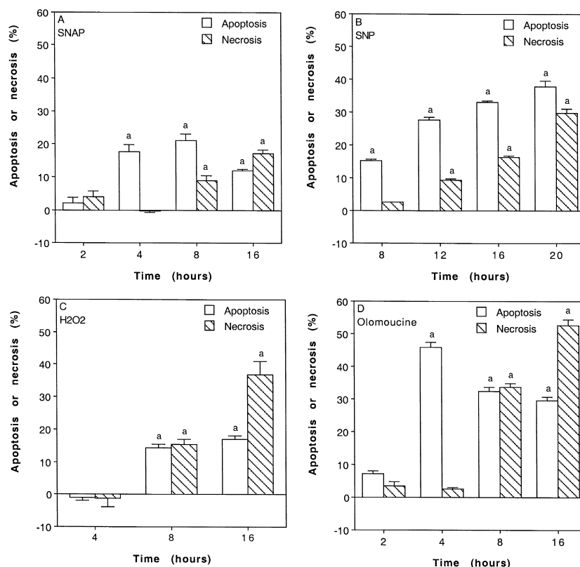
Fig. 3. Time dependent effect of 0.5 mM S -nitroso- N -acetylpenicillamine, 2 mM sodium nitroprusside, 0.5 mM H 2 O 2 and 0.2 mM olomoucine on apoptosis and necrosis in CHP212 cells. Data represent means \pm S.E.M. of triplicate determinations. a Indicates a significant difference from control ( P < 0.05 ).
